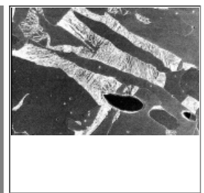
Figure 4. A scanning electron micrograph of the etched surface of the Titanic hull steel showing pearlite colonies, ferrite grains, an elongated MnS particle, and nonmetallic inclusions. Etchant is 2% Nital.
