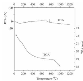
Figure 2. TGA and DTA of co-precipitated samarium, holmium and iron hydroxides with composition Sm 0.6 Ho 2.4 Fe 10 O 24 in air, with heating rate of 10 °C/min.
