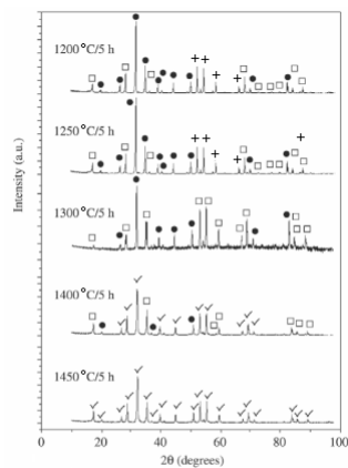
Figure 4. X-ray diffraction pattern of the ceramic pieces sintered at different temperatures in the 1200 to 1450 °C range, where \bullet \text{Sm}_3\text{Fe}_5\text{O}_{12} , \square \text{Ho}_3\text{Fe}_5\text{O}_{12} , \checkmark \text{Sm}_6\text{Ho}_2\text{Fe}_9\text{O}_{12} and + \text{SmFeO}_3 .
