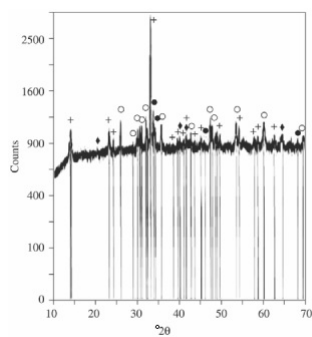
Figure 3. X-ray diffraction pattern of the samarium, holmium, iron co precipitate after calcination at 1000 °C, where + \text{HoFeO}_3 , \circ \text{Sm}_2\text{O}_3 and \blacklozenge \text{Ho}_2\text{O}_3 .
